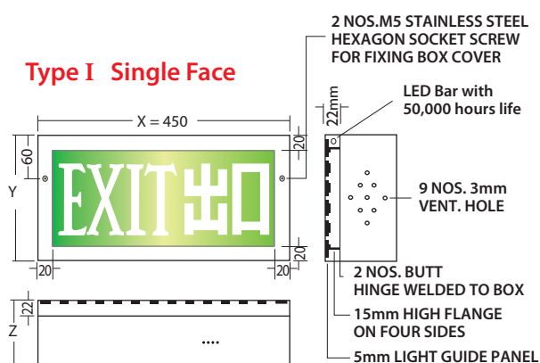
"CRYSTALITE" Cat. CX-LED-8-B-I-DC
