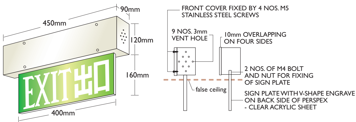
"CRYSTALITE" Cat. CX-8-P 1x8W, emergency exit sign plate
